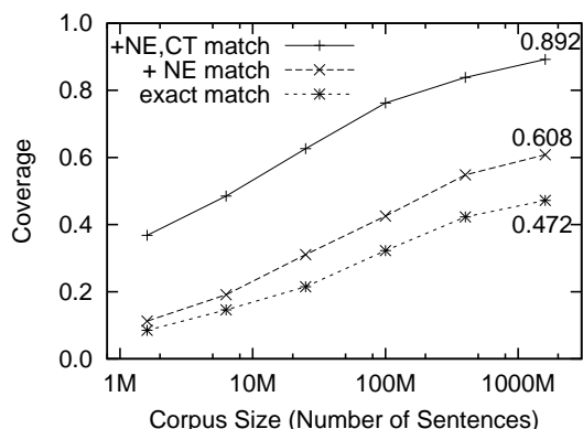
Figure 2: Coverage of CF (omitted argument).
