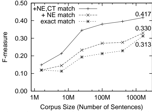
Figure 6: F-measure of Zero Anaphora Resolution.
