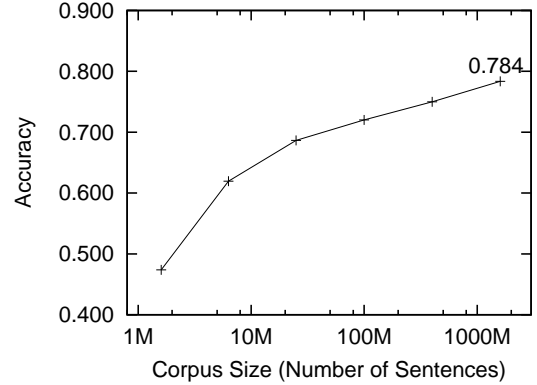
Figure 5: Accuracy of Case Structure Analysis.
