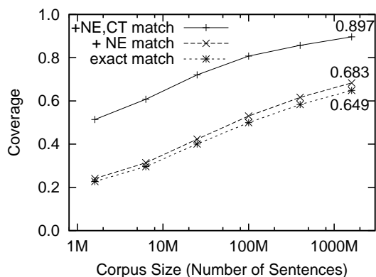
Figure 1: Coverage of CF (overt argument).
